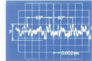
Discharge Pressure Variation in a 3-Lobes Rotor
