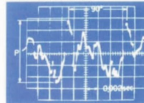
Discharge Pressure Variation in a 2-Lobes Rotor
